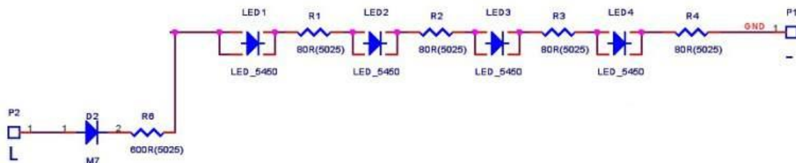
Circuit diagram
